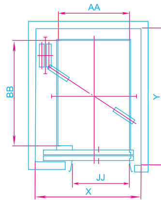
Oil Hydraulic Cargo Lift
