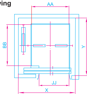
Rope Cable Cargo Lift
